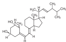
Figure 1: Chemical Structure of Doxercalciferol
